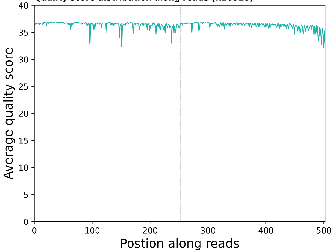
Quality score distribution along reads (R10528)
